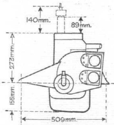
60 h.p. two-stroke Caunter C.
