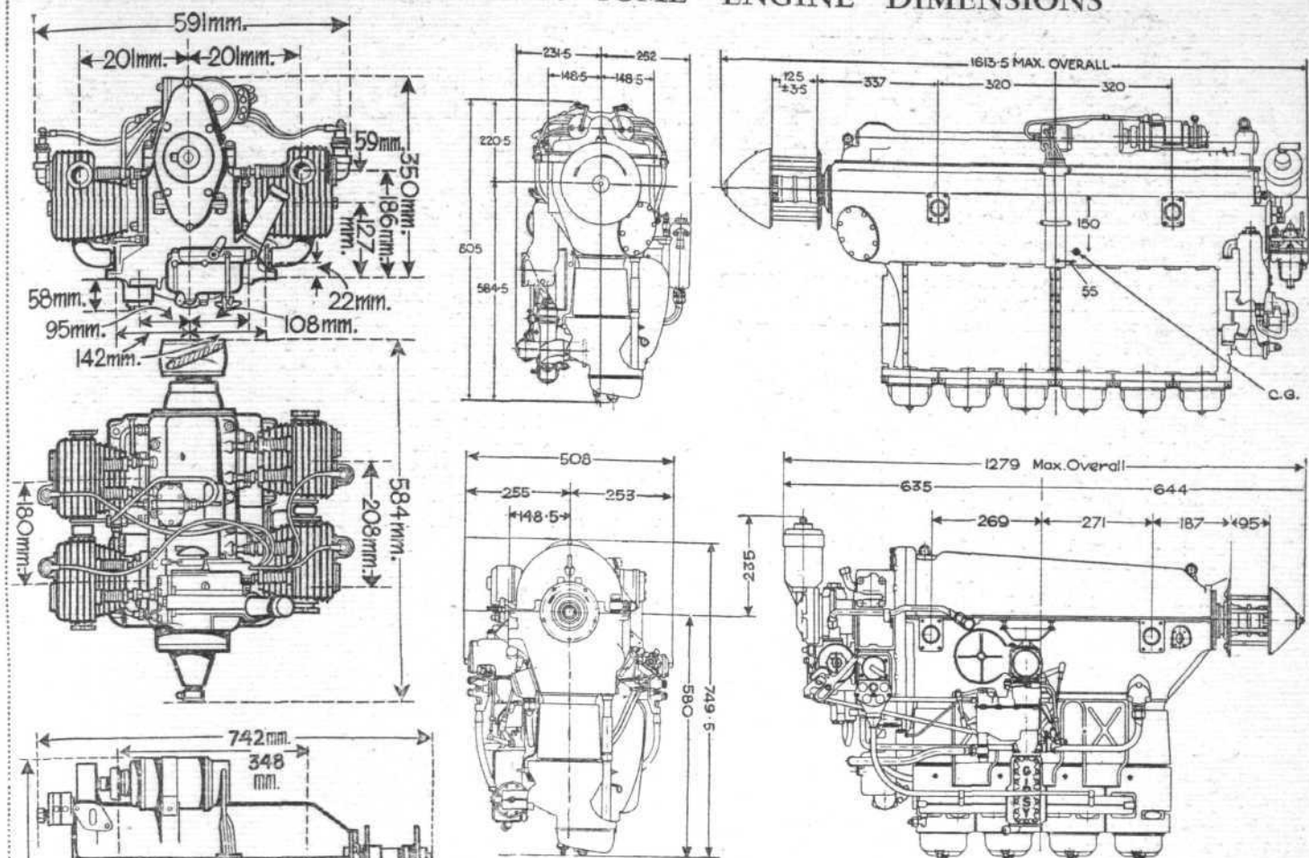
(Top right) The 205 h.p. Gipsy Six Series II and, below it, the 140 h.p. Gipsy Major II; both these engines can drive the 1,000 size D.H. v.p. airscrew. (Top left) The four-cylinder 40 h.p. Coventry Victor Neptune III.
