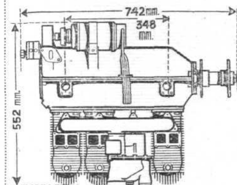
60 h.p. two-stroke Caunter C.
